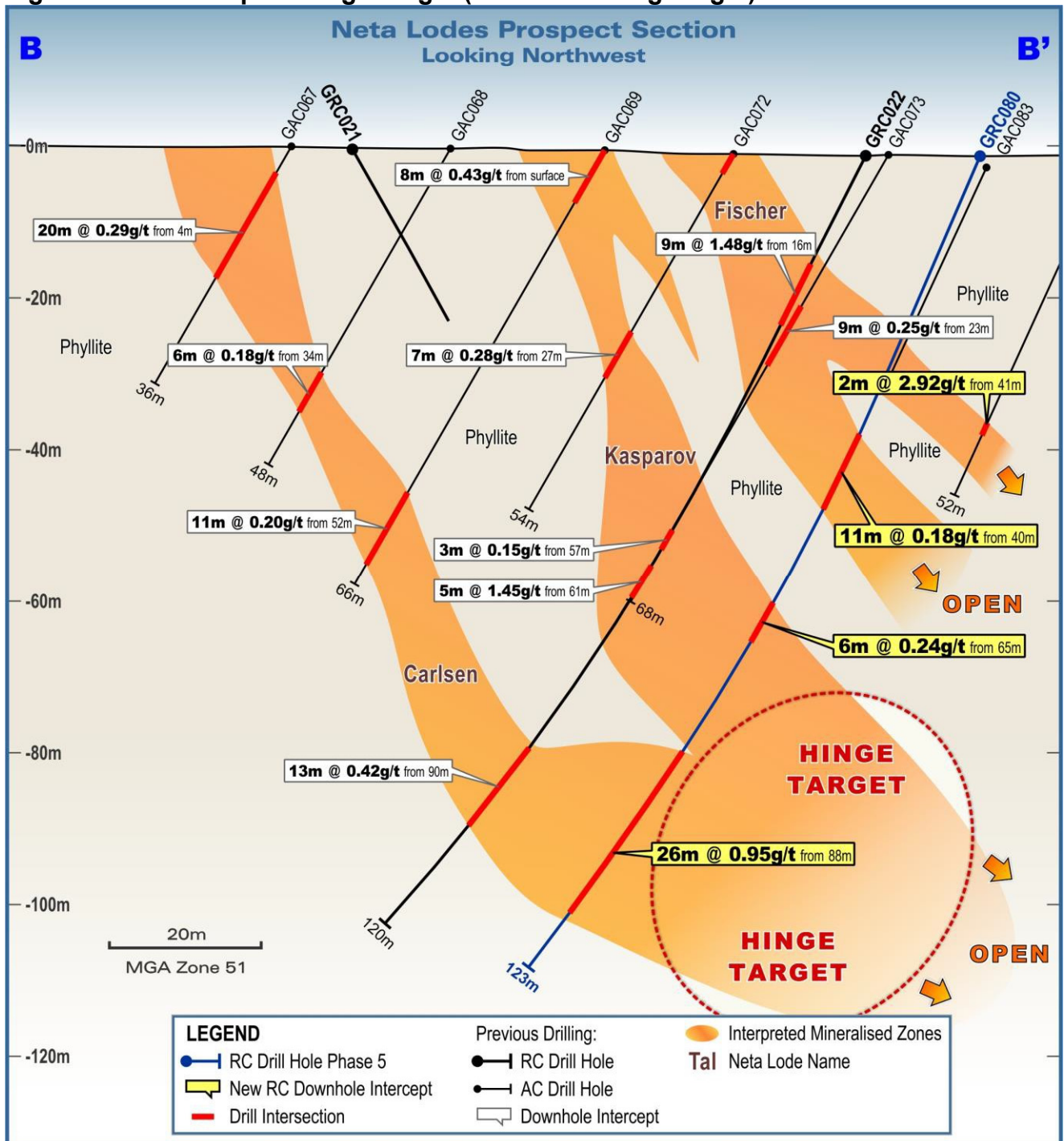
Figure 2: Neta Prospect Hinge Target (Phase 7 Drilling Target)
